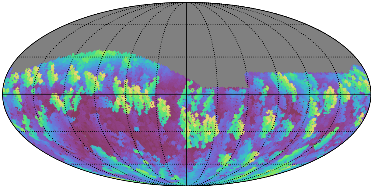
scp_reweight_v3.3_10yrs Yr 1 z band: Max airmass
