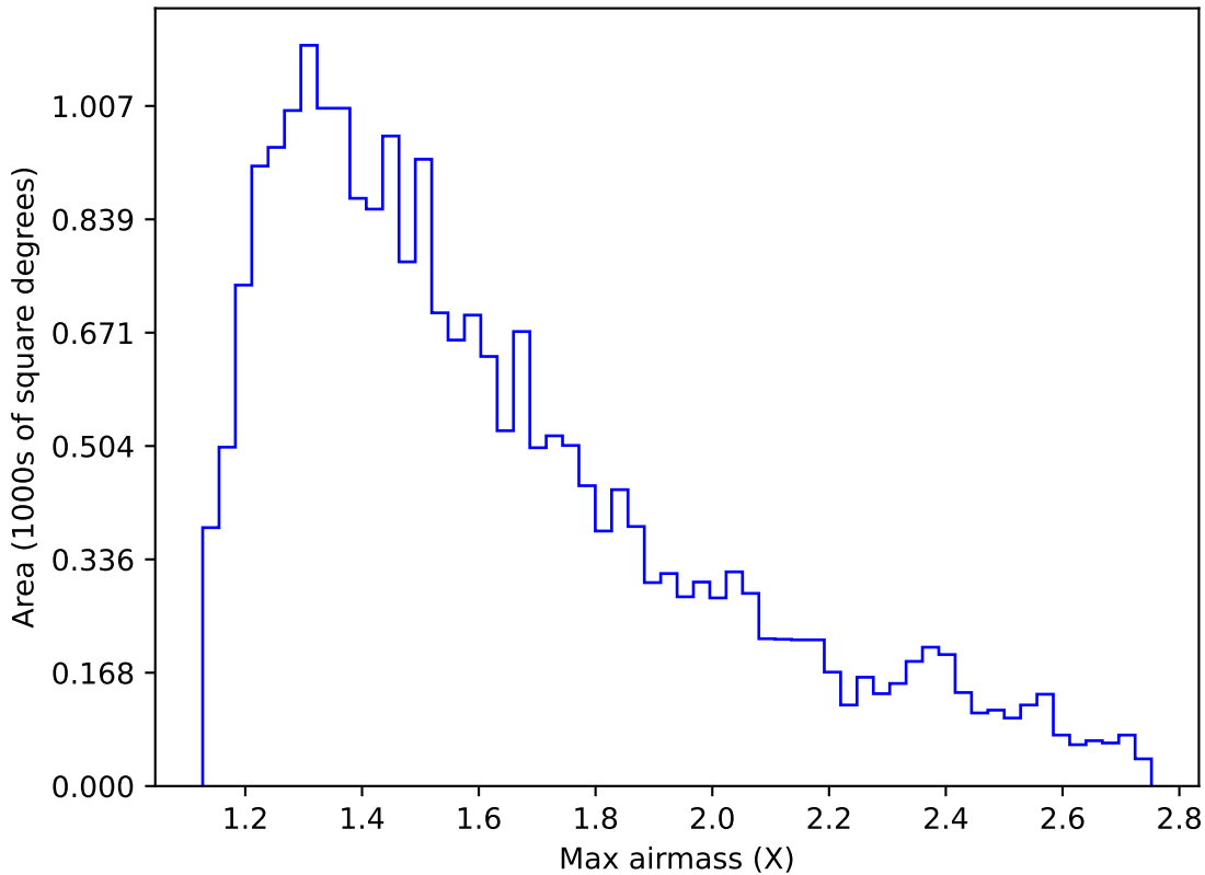
scp_reweight_v3.3_10yrs Yr 1 y band: Max airmass
