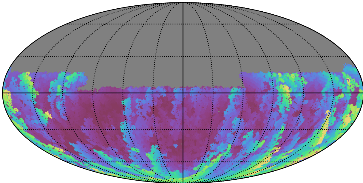
scp_reweight_v3.3_10yrs Yr 1 u band: Max airmass
