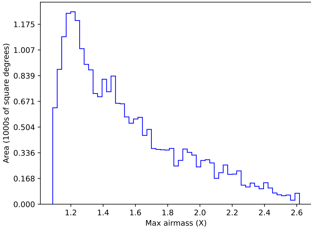
scp_reweight_v3.3_10yrs Yr 1 u band: Max airmass
