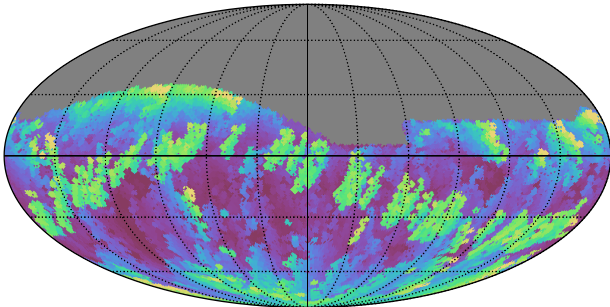
scp_reweight_v3.3_10yrs Yr 1 r band: Max airmass
