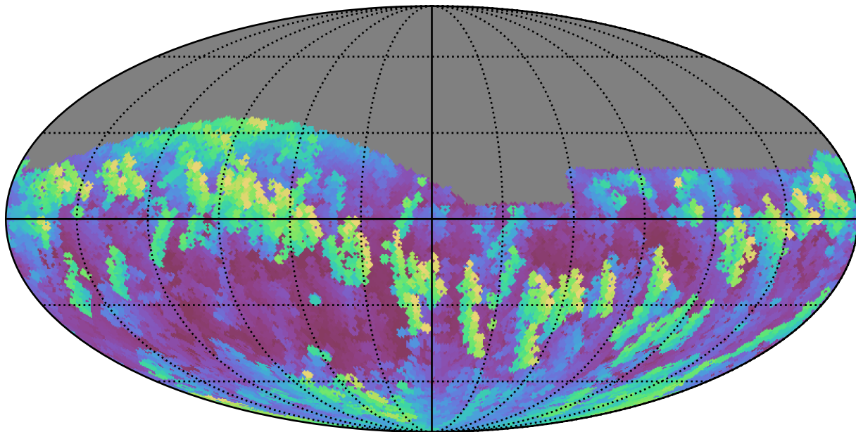
scp_reweight_v3.3_10yrs Yr 1 i band: Max airmass
