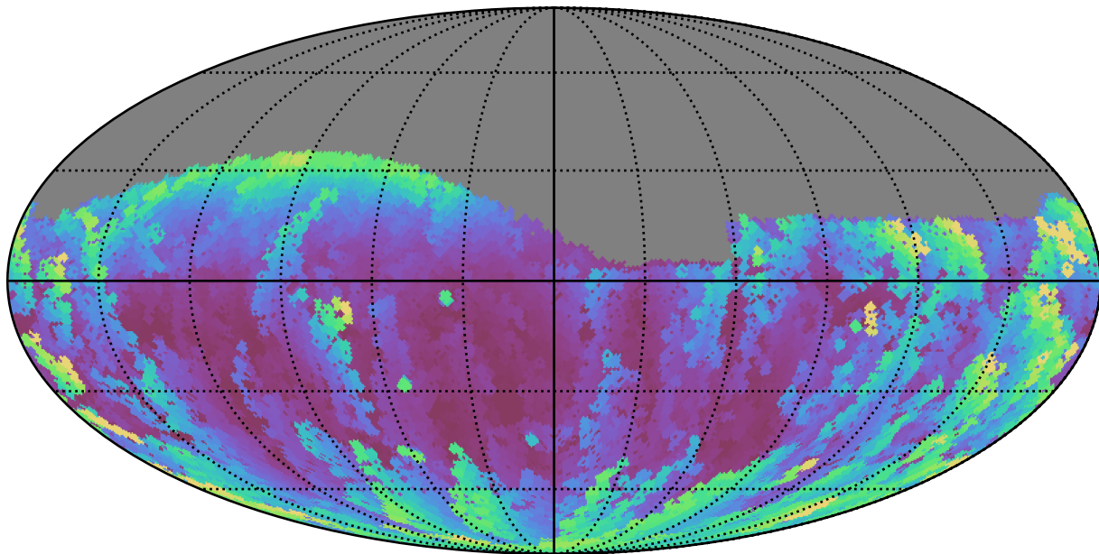
scp_reweight_v3.3_10yrs Yr 1 g band: Max airmass
