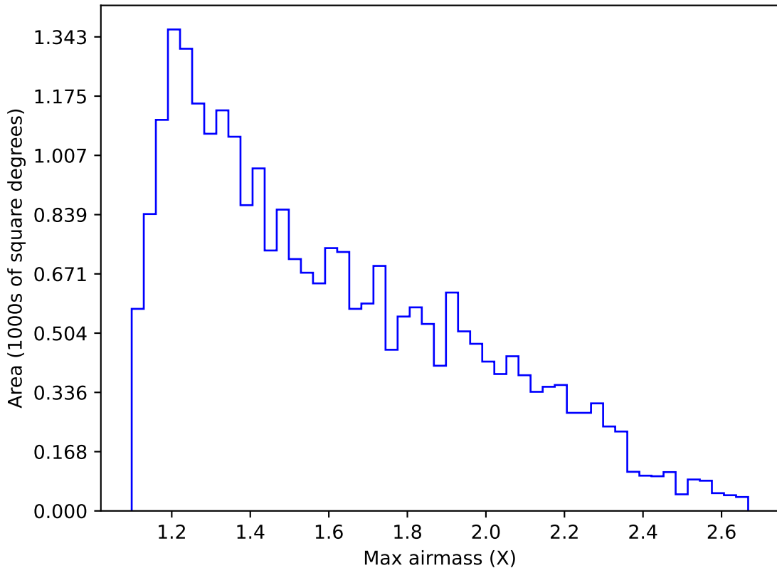
scp_reweight_v3.3_10yrs Yr 1 g band: Max airmass
