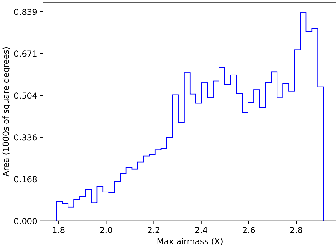
scp_reweight_v3.3_10yrs WFD z band: Max airmass
