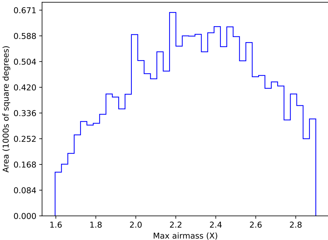
scp_reweight_v3.3_10yrs WFD y band: Max airmass
