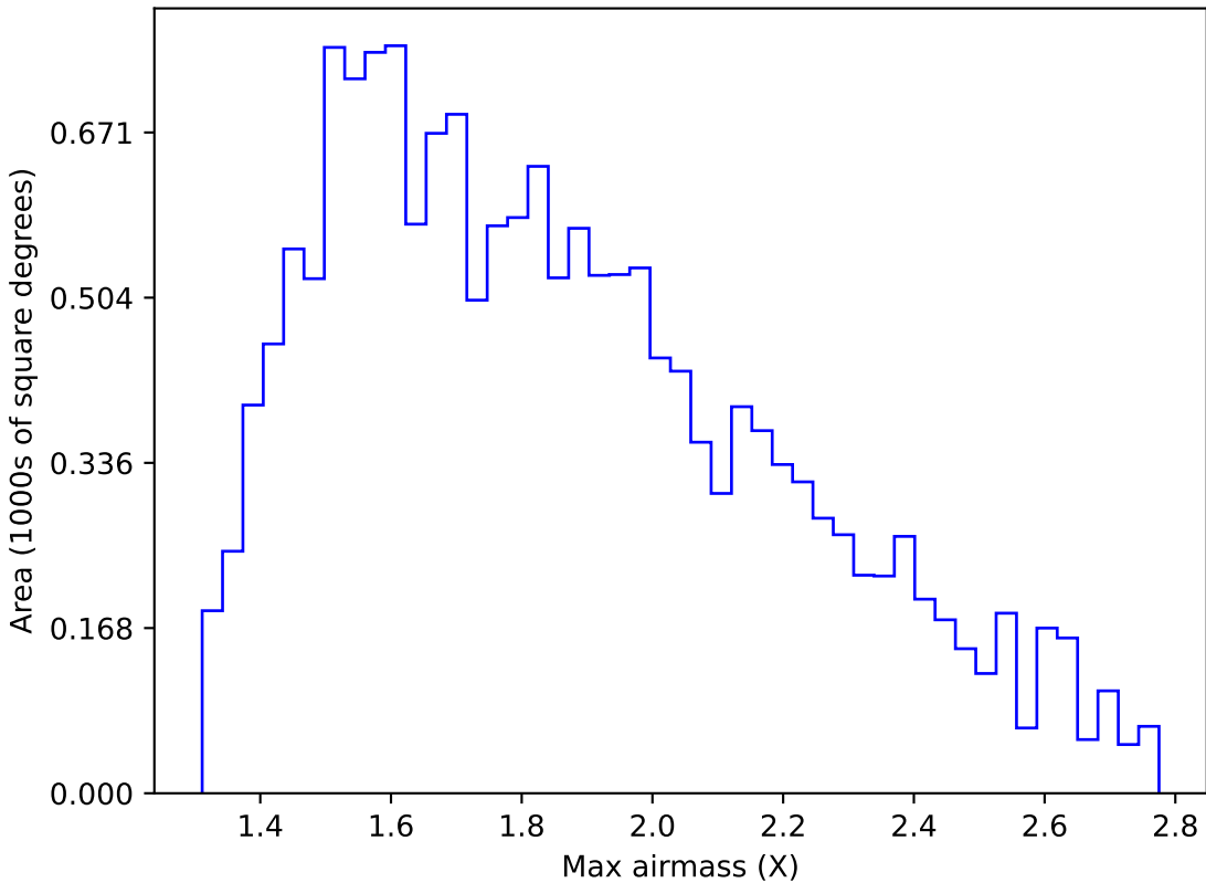
scp_reweight_v3.3_10yrs WFD u band: Max airmass
