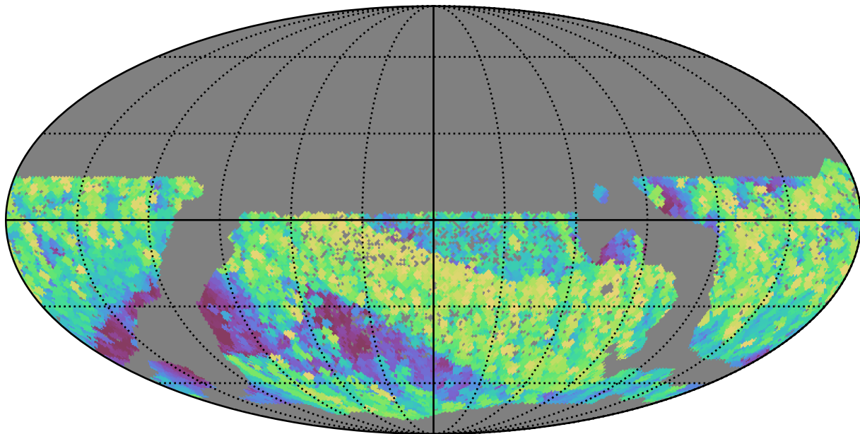
scp_reweight_v3.3_10yrs WFD i band: Max airmass
