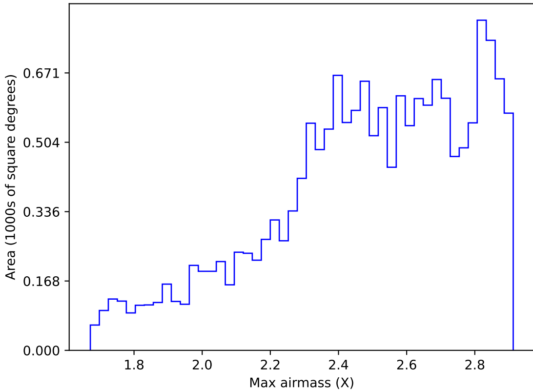
scp_reweight_v3.3_10yrs WFD i band: Max airmass
