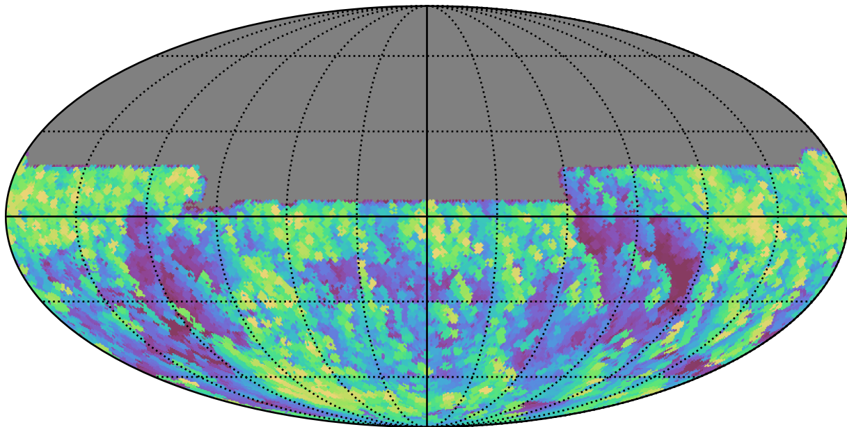
scp_reweight_v3.3_10yrs All sky y band: Max airmass
