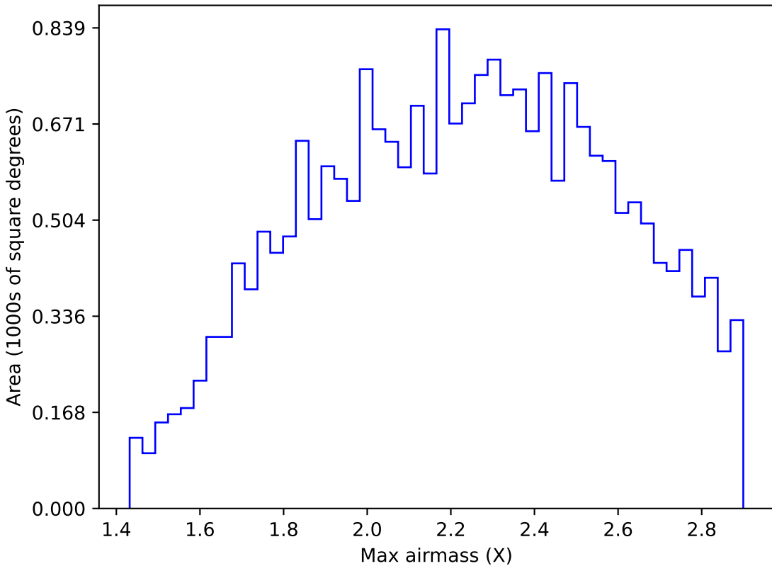
scp_reweight_v3.3_10yrs All sky y band: Max airmass
