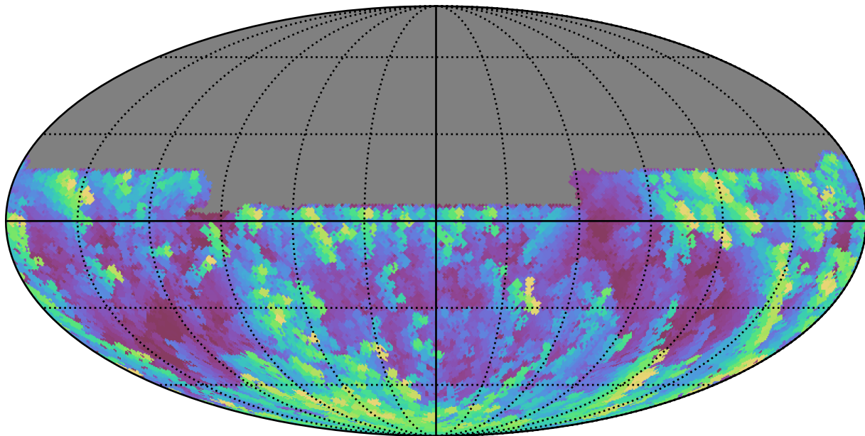
scp_reweight_v3.3_10yrs All sky u band: Max airmass
