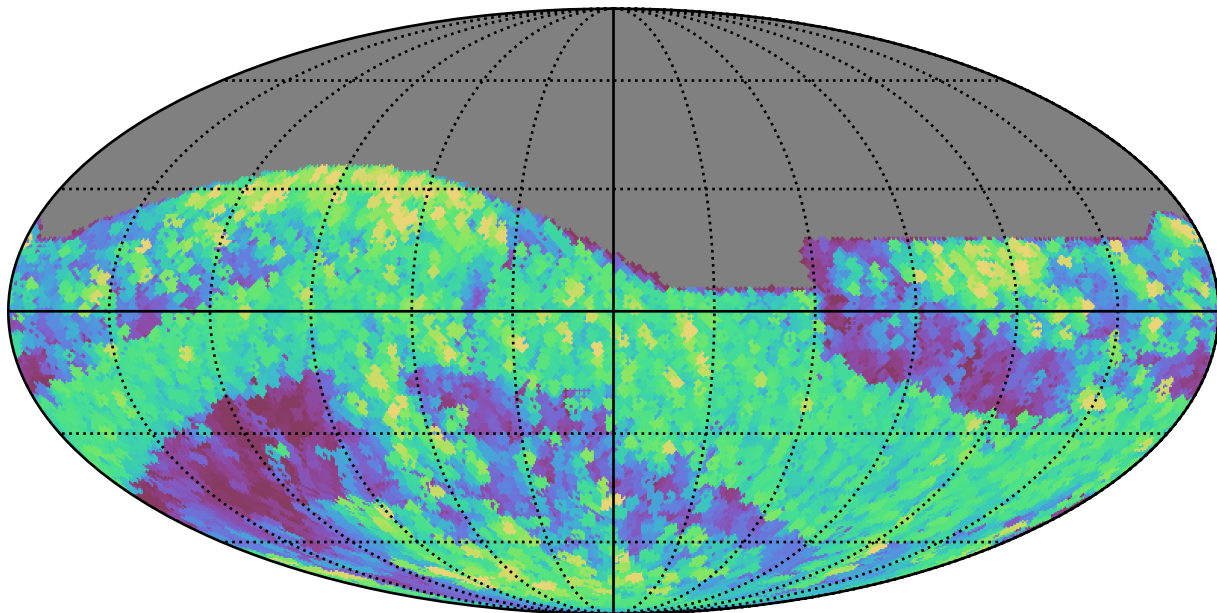
scp_reweight_v3.3_10yrs All sky r band: Max airmass
