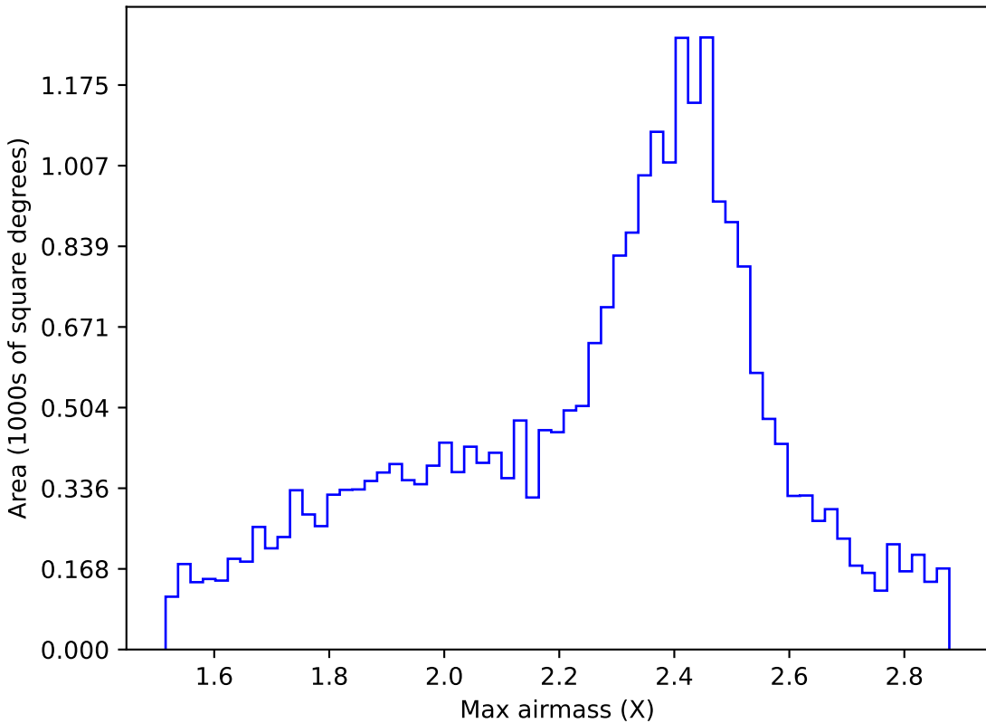
scp_reweight_v3.3_10yrs All sky r band: Max airmass
