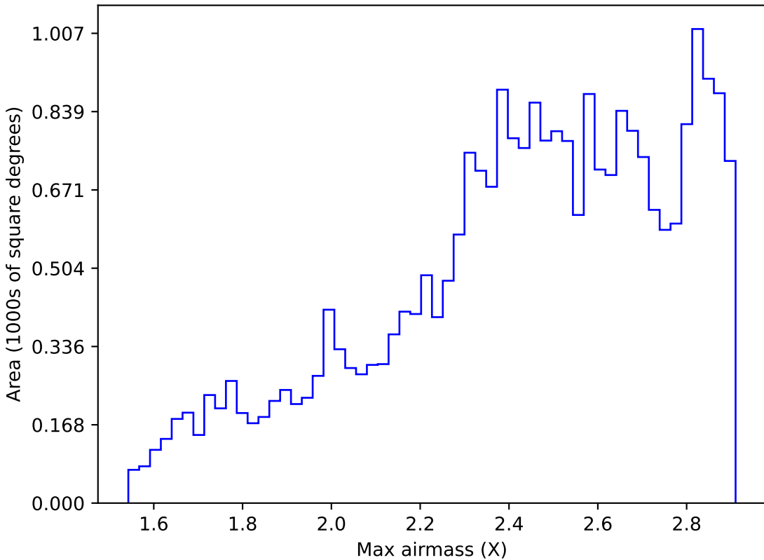
scp_reweight_v3.3_10yrs All sky i band: Max airmass
