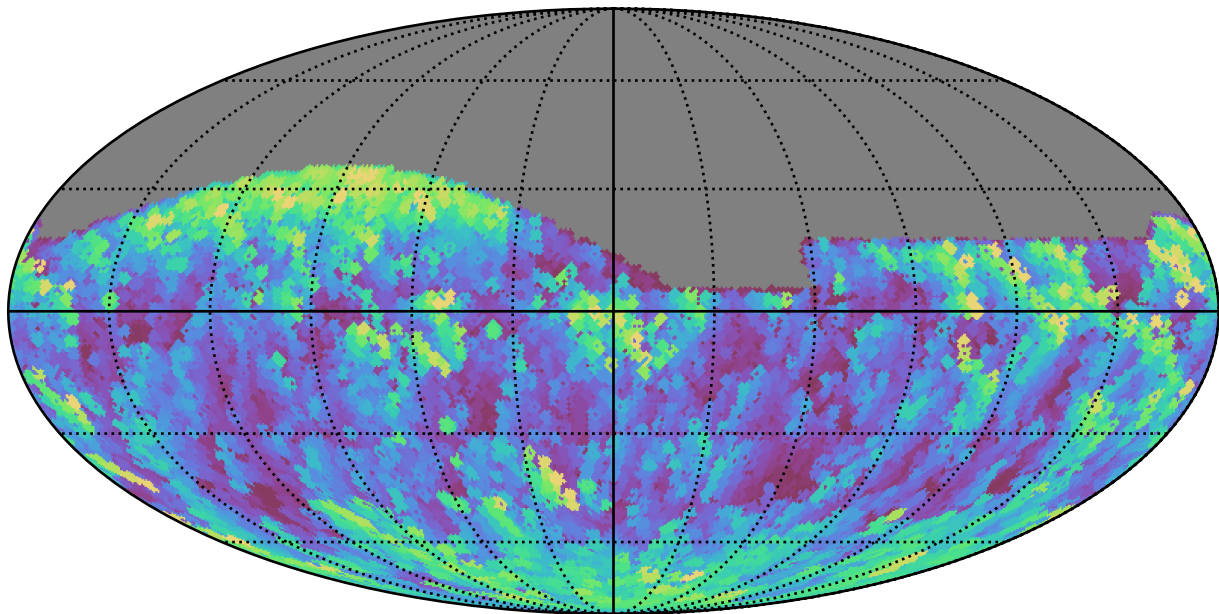
scp_reweight_v3.3_10yrs All sky g band: Max airmass
