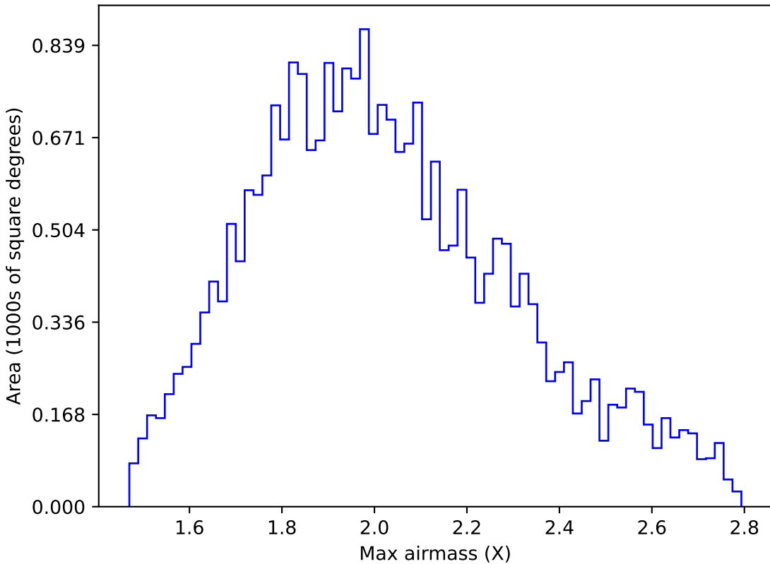
scp_reweight_v3.3_10yrs All sky g band: Max airmass
