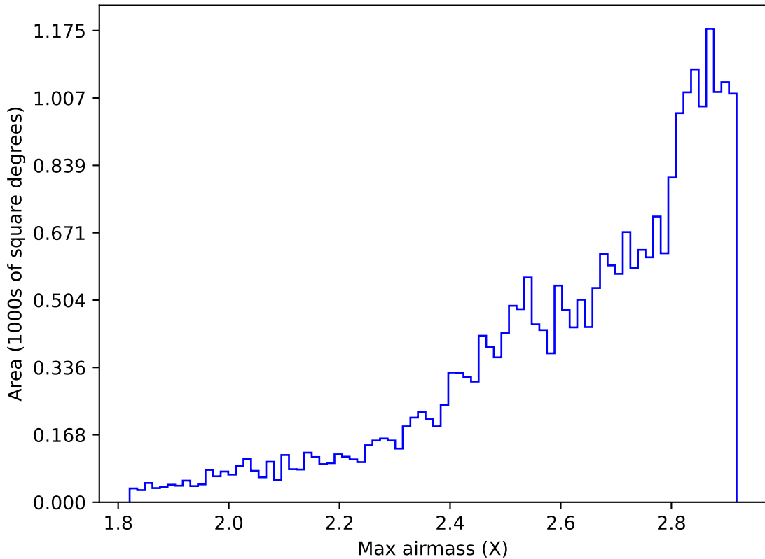
scp_reweight_v3.3_10yrs All sky all bands: Max airmass
