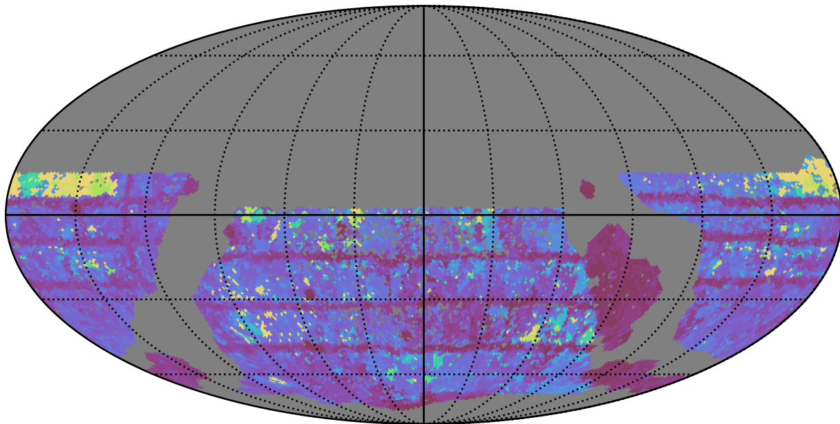
scp_reweight_v3.3_10yrs WFD z band: Max Inter-Night Gap
