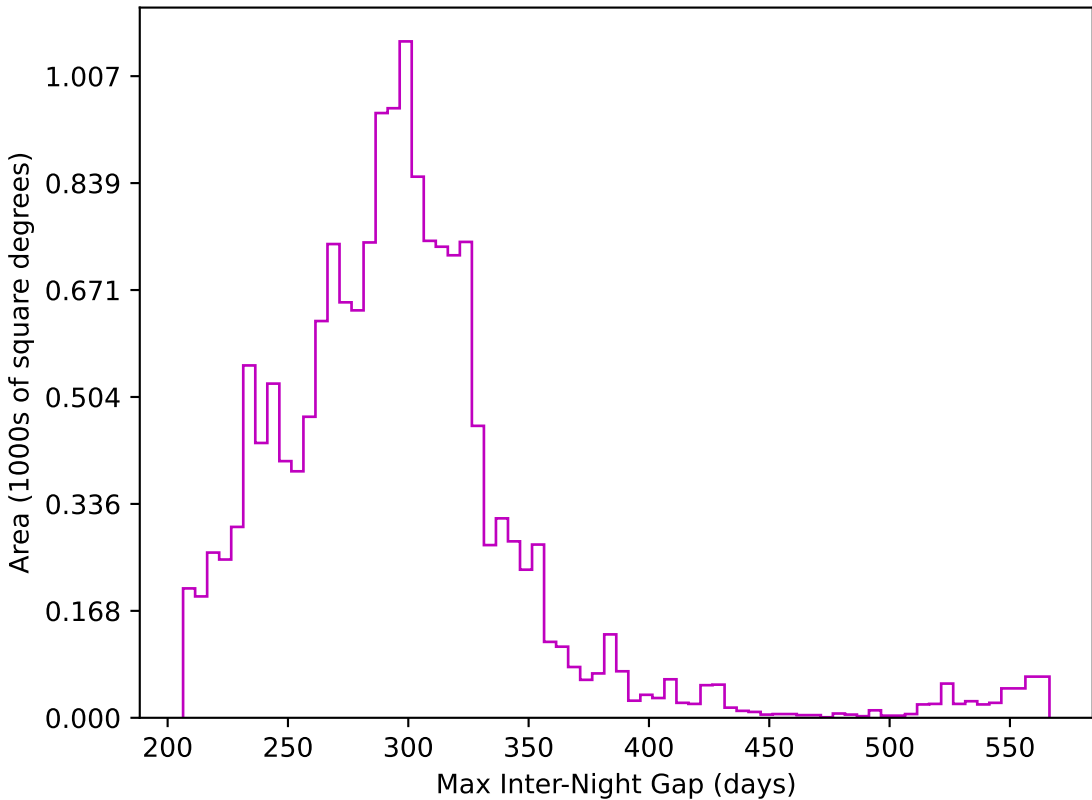
scp_reweight_v3.3_10yrs WFD z band: Max Inter-Night Gap
