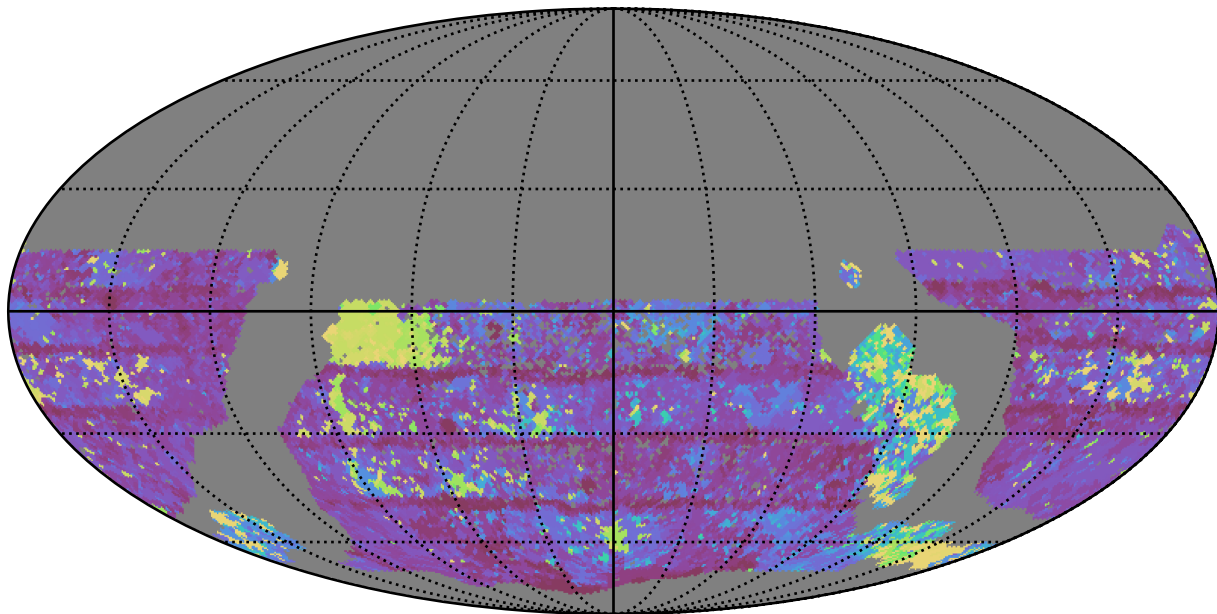
scp_reweight_v3.3_10yrs WFD y band: Max Inter-Night Gap
