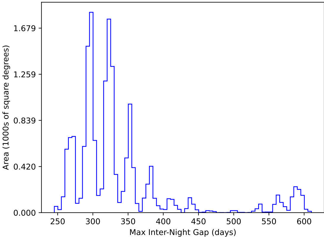
scp_reweight_v3.3_10yrs WFD y band: Max Inter-Night Gap
