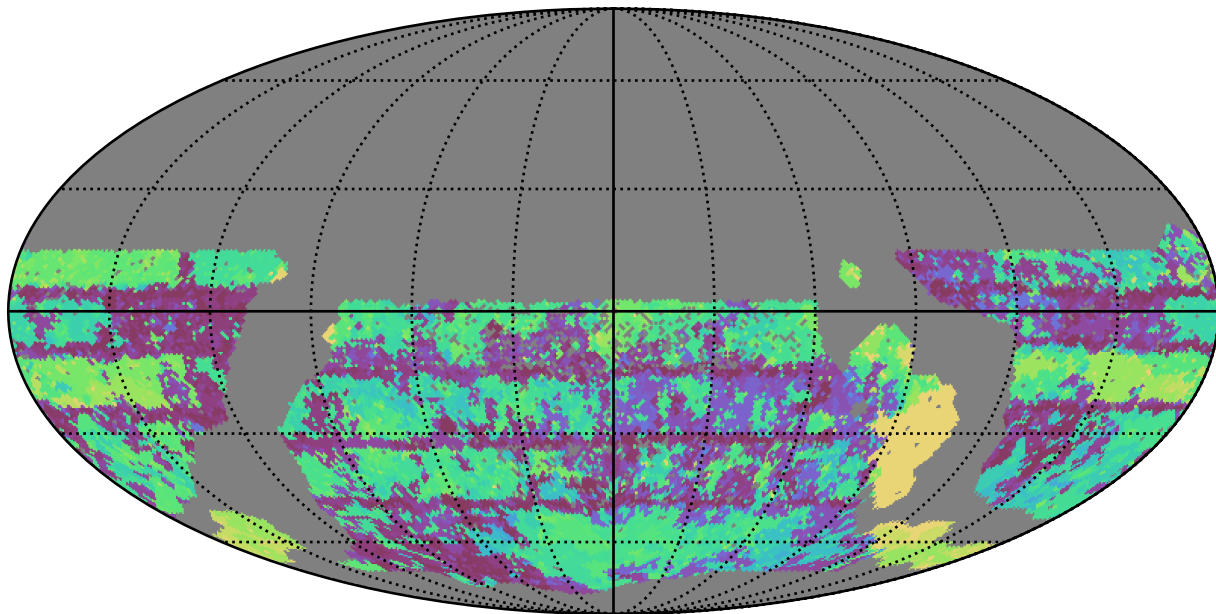
scp_reweight_v3.3_10yrs WFD u band: Max Inter-Night Gap
