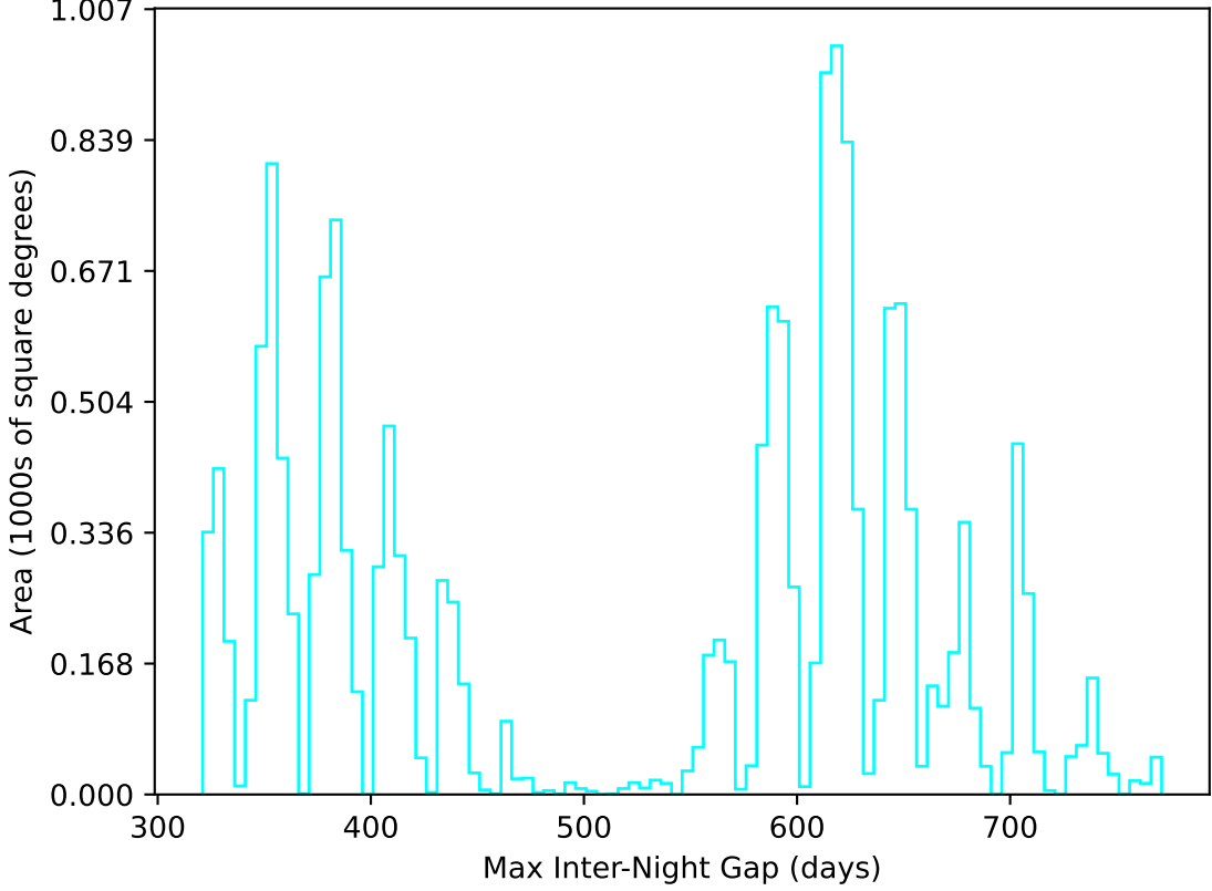
scp_reweight_v3.3_10yrs WFD u band: Max Inter-Night Gap
