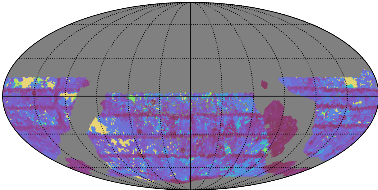
scp_reweight_v3.3_10yrs WFD i band: Max Inter-Night Gap
