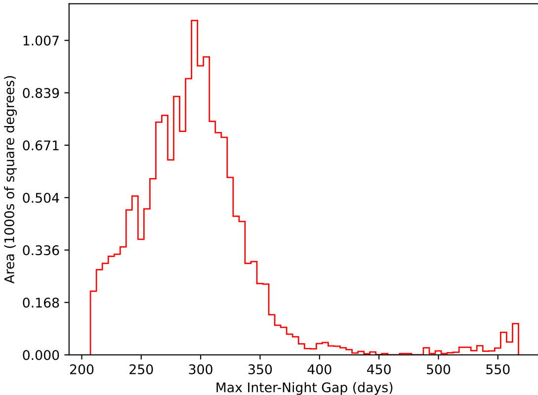
scp_reweight_v3.3_10yrs WFD i band: Max Inter-Night Gap
