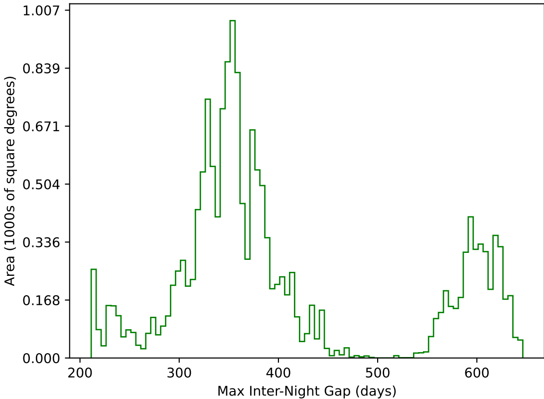
scp_reweight_v3.3_10yrs WFD g band: Max Inter-Night Gap
