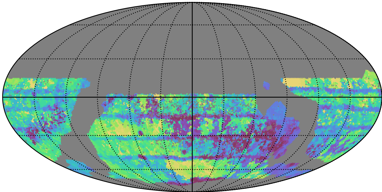
scp_reweight_v3.3_10yrs WFD all bands: Max Inter-Night Gap
