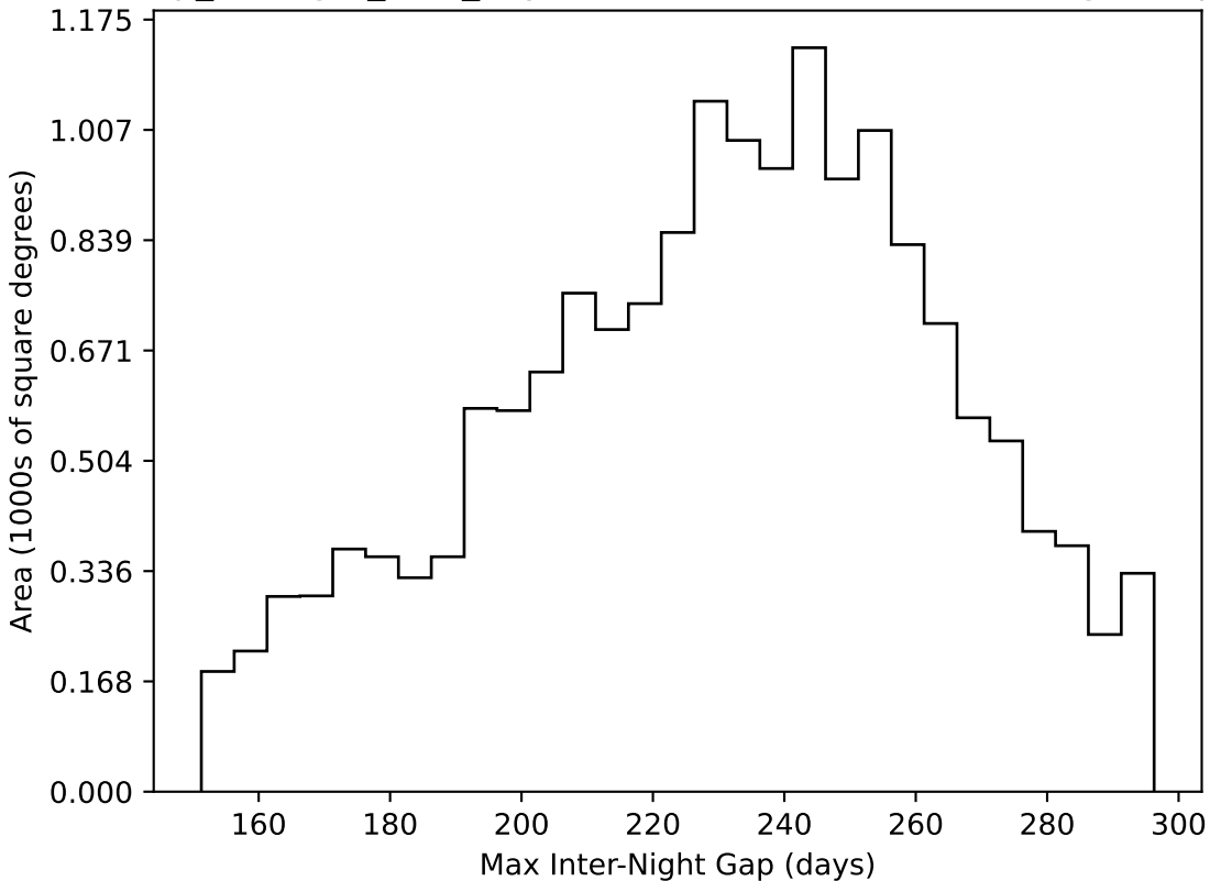
scp_reweight_v3.3_10yrs WFD all bands: Max Inter-Night Gap
