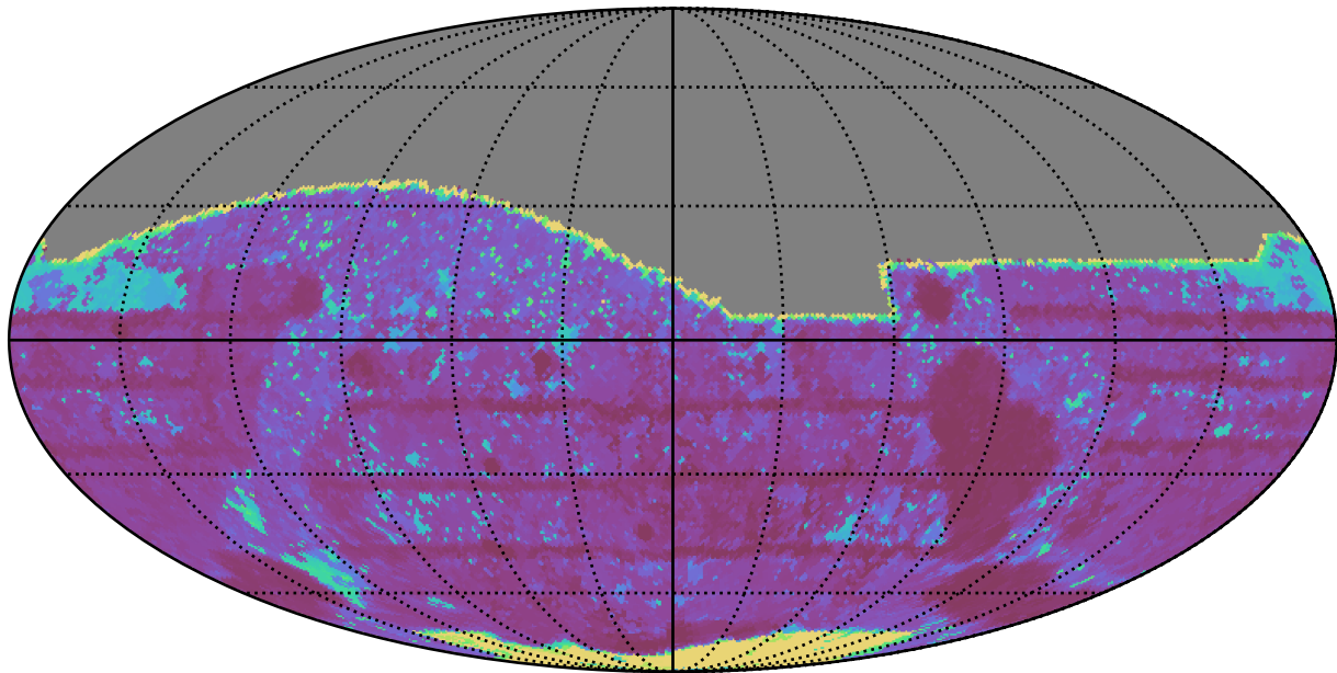
scp_reweight_v3.3_10yrs All sky z band: Max Inter-Night Gap
