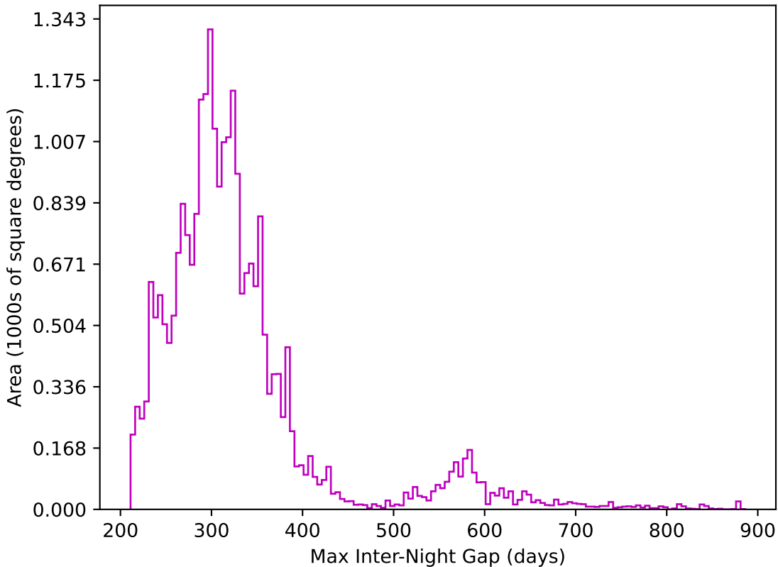
scp_reweight_v3.3_10yrs All sky z band: Max Inter-Night Gap
