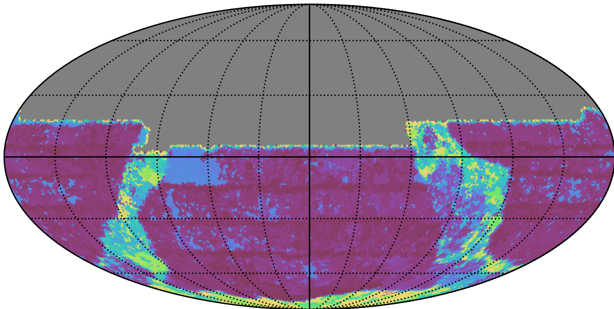
scp_reweight_v3.3_10yrs All sky y band: Max Inter-Night Gap
