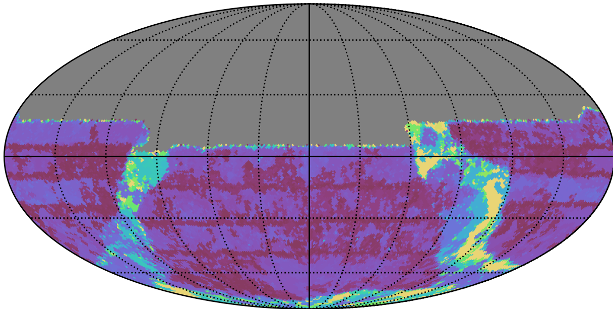
scp_reweight_v3.3_10yrs All sky u band: Max Inter-Night Gap
