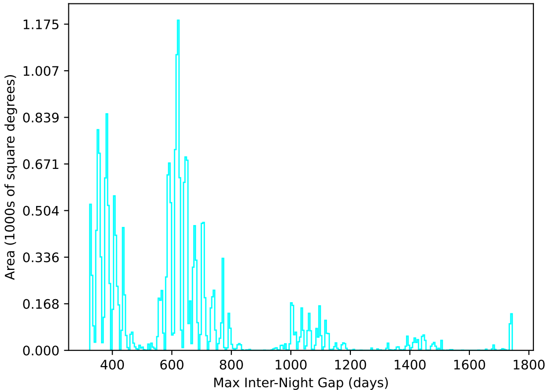
scp_reweight_v3.3_10yrs All sky u band: Max Inter-Night Gap
