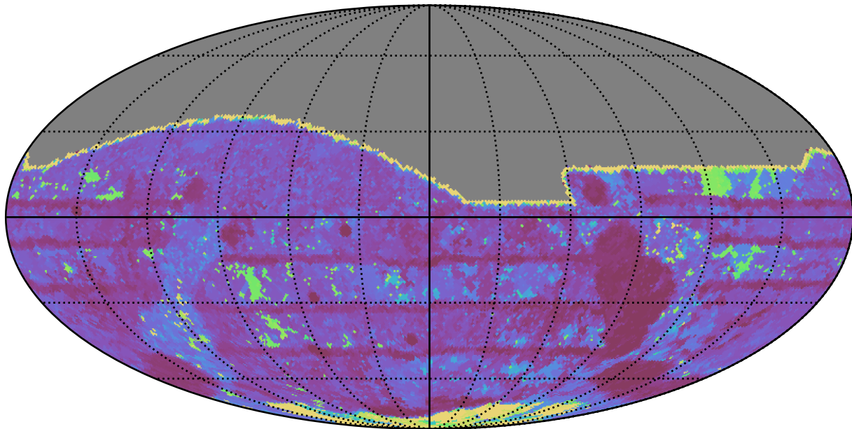
scp_reweight_v3.3_10yrs All sky r band: Max Inter-Night Gap
