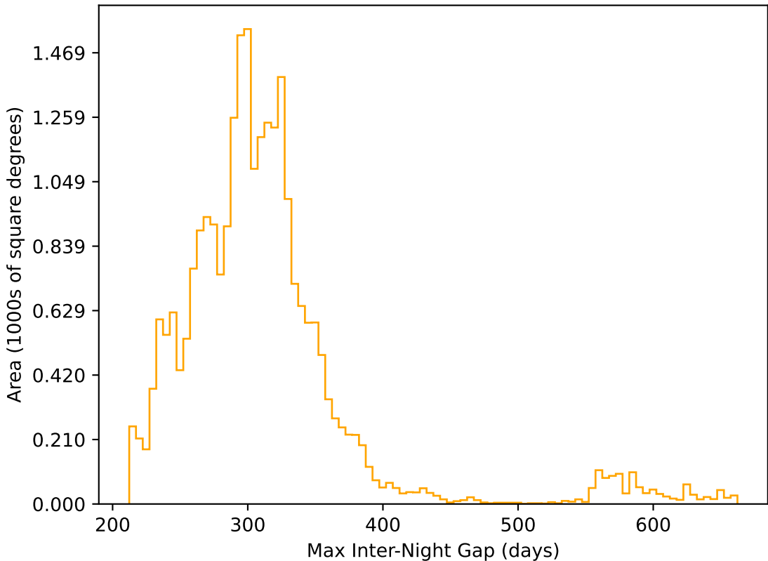
scp_reweight_v3.3_10yrs All sky r band: Max Inter-Night Gap
