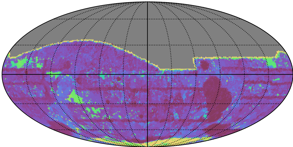
scp_reweight_v3.3_10yrs All sky i band: Max Inter-Night Gap
