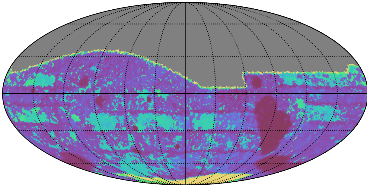
scp_reweight_v3.3_10yrs All sky g band: Max Inter-Night Gap
