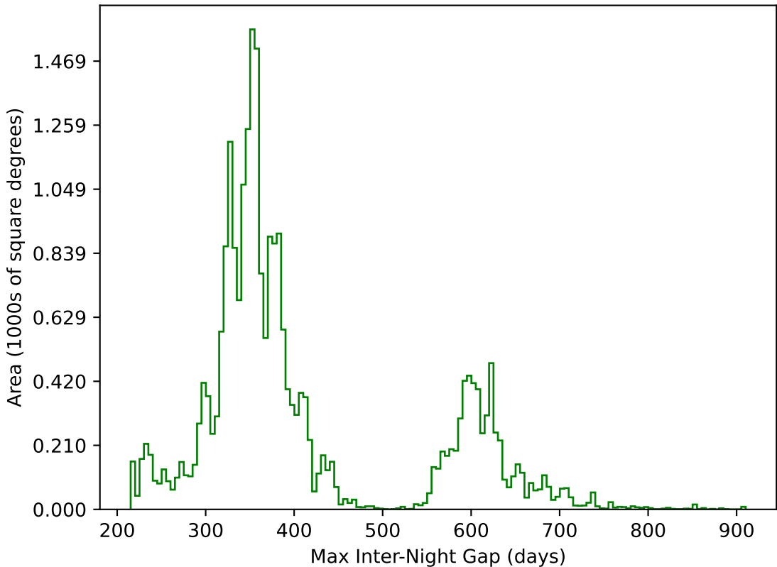
scp_reweight_v3.3_10yrs All sky g band: Max Inter-Night Gap
