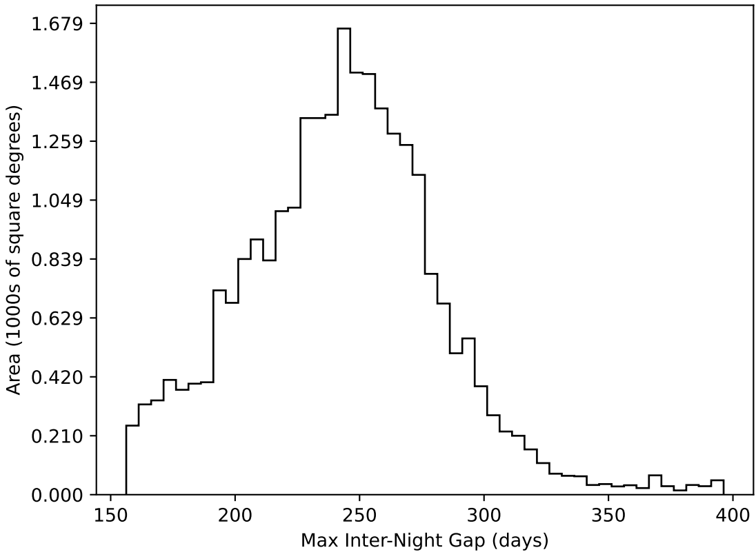
scp_reweight_v3.3_10yrs All sky all bands: Max Inter-Night Gap
