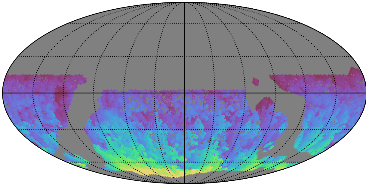
scp_reweight_v3.3_10yrs WFD y band: Max HA
