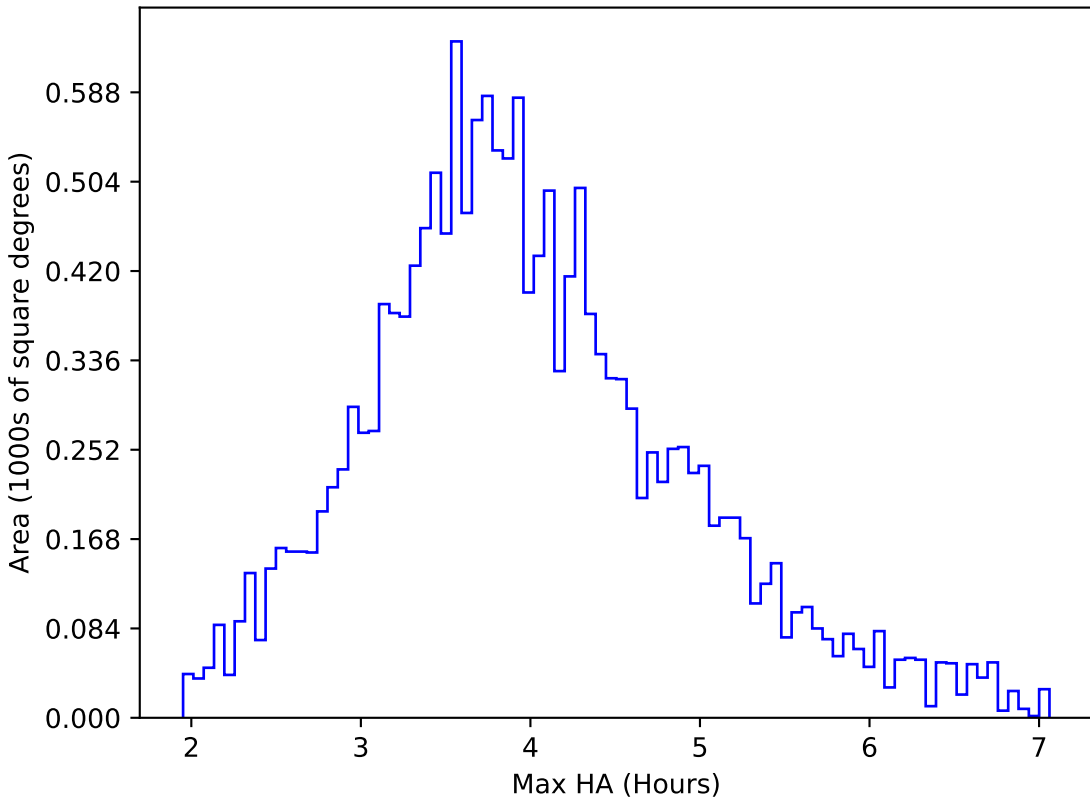
scp_reweight_v3.3_10yrs WFD u band: Max HA
