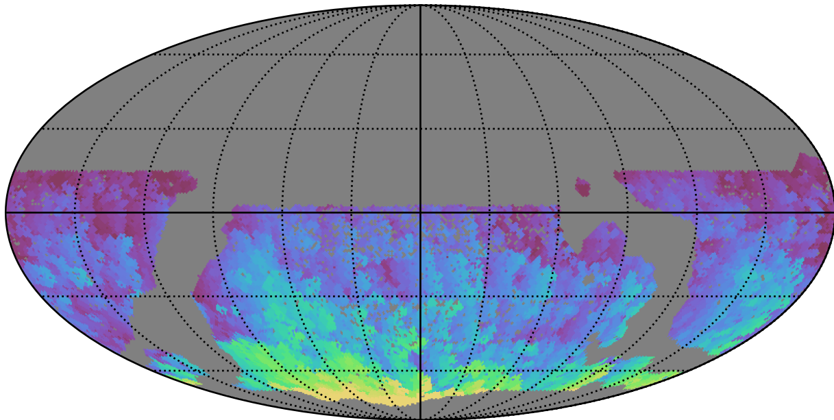
scp_reweight_v3.3_10yrs WFD r band: Max HA
