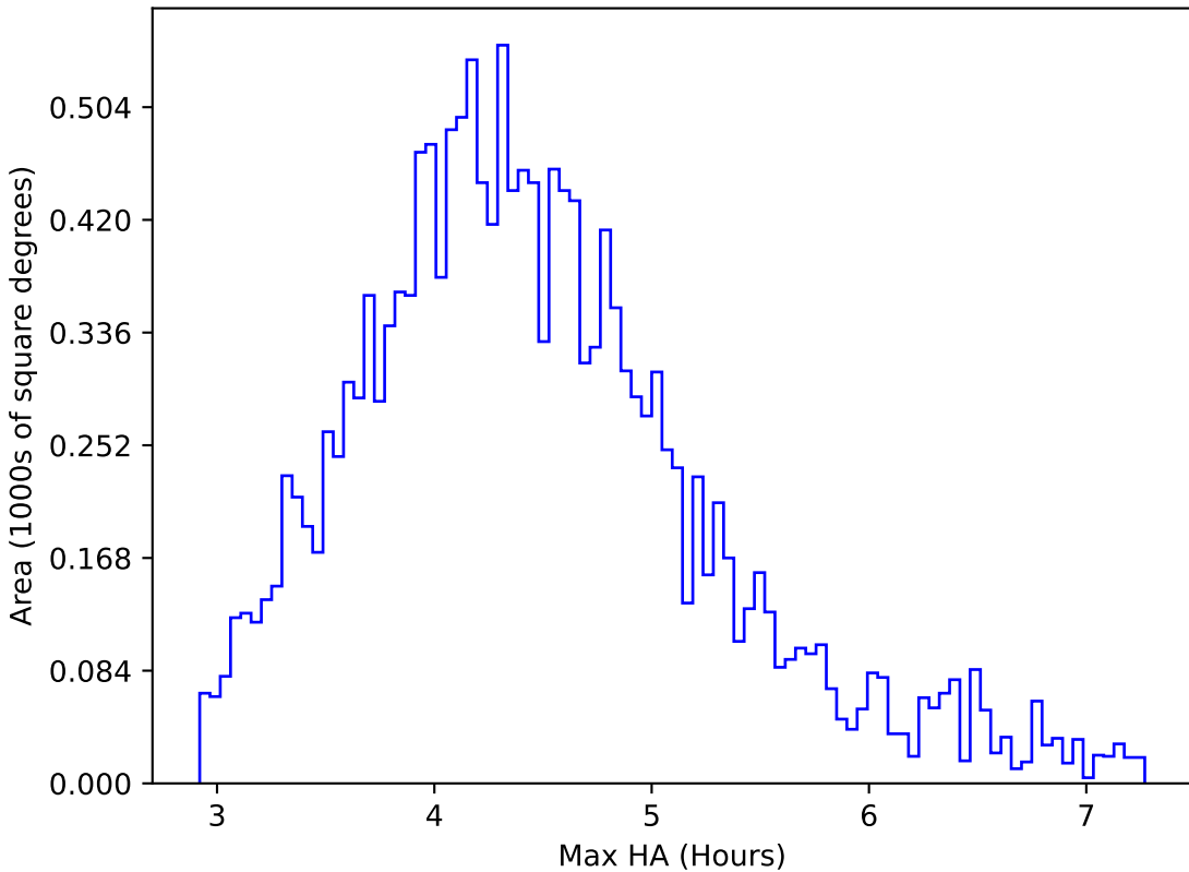
scp_reweight_v3.3_10yrs WFD r band: Max HA
