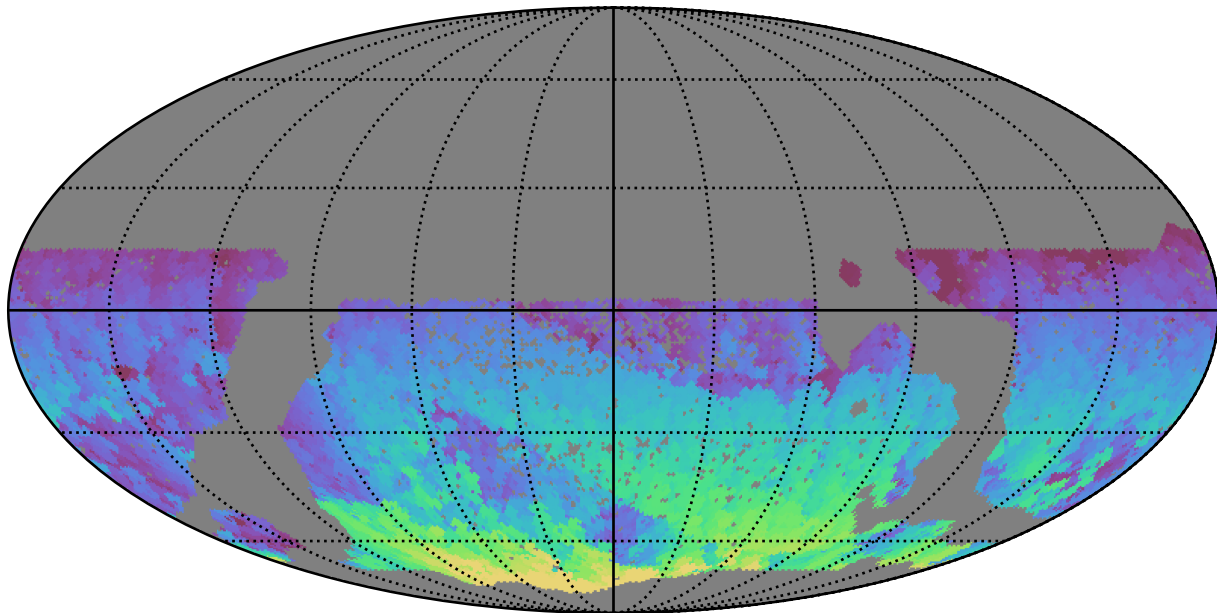
scp_reweight_v3.3_10yrs WFD i band: Max HA
