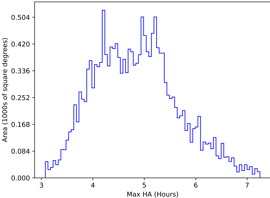
scp_reweight_v3.3_10yrs WFD i band: Max HA
